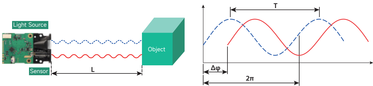
Figure 1-1 Basic Schematic Diagram of Laser Module
